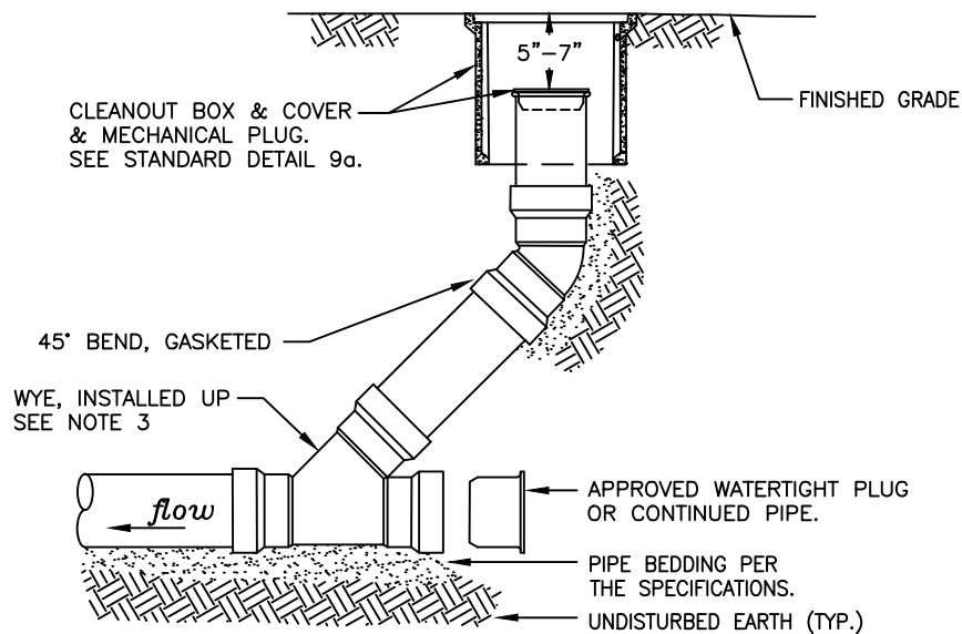
WYE CLEANOUT (INSIDE PROPERTY) PROFILE
