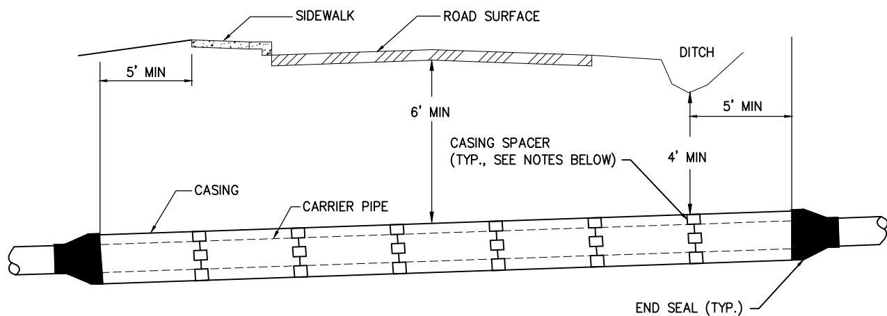
ROADWAY SECTION
