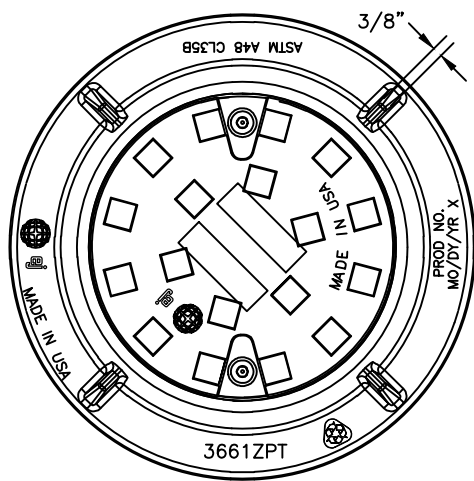
COVER AND FRAME PLAN
