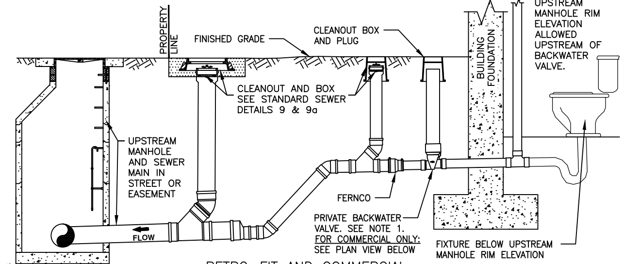
RETRO-FIT AND COMMERCIAL PROFILE (OUTSIDE BACKFLOW VALVE)
