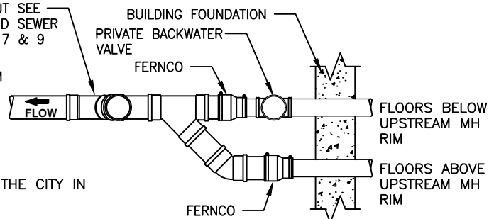
COMMERCIAL PLAN (FOR OUTSIDE BACKWATER VALVE)
