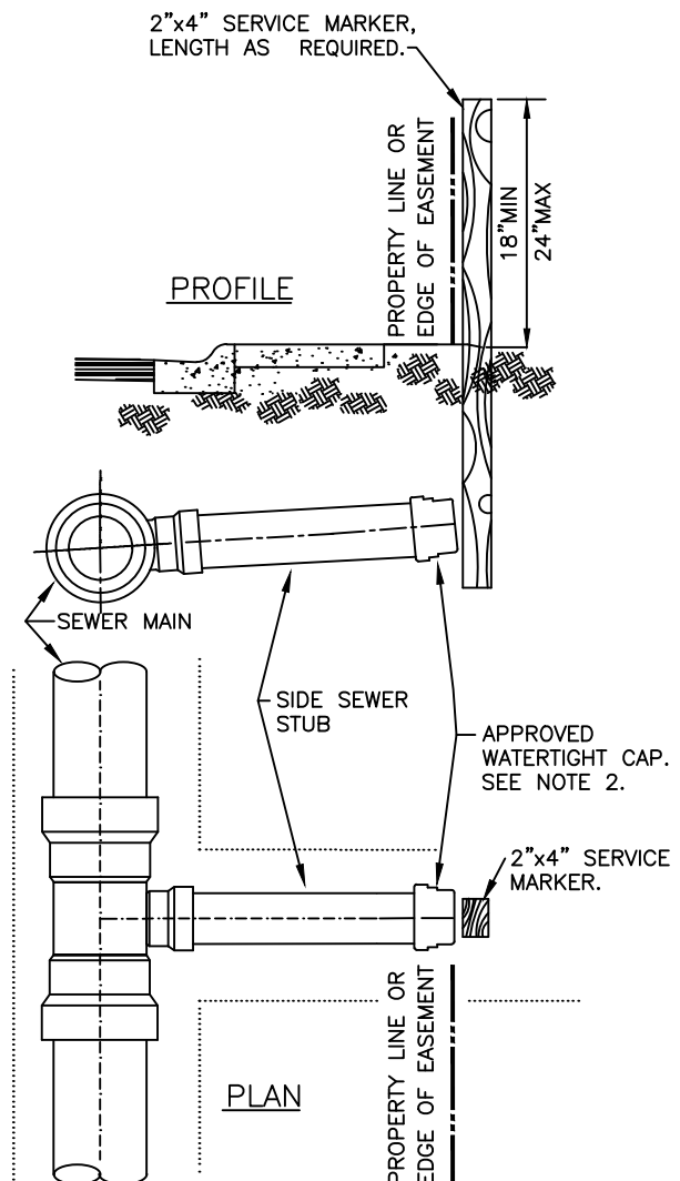
TEMPORARY ABANDONMENT
