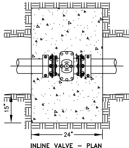
INLINE VALVE — PROFILE
